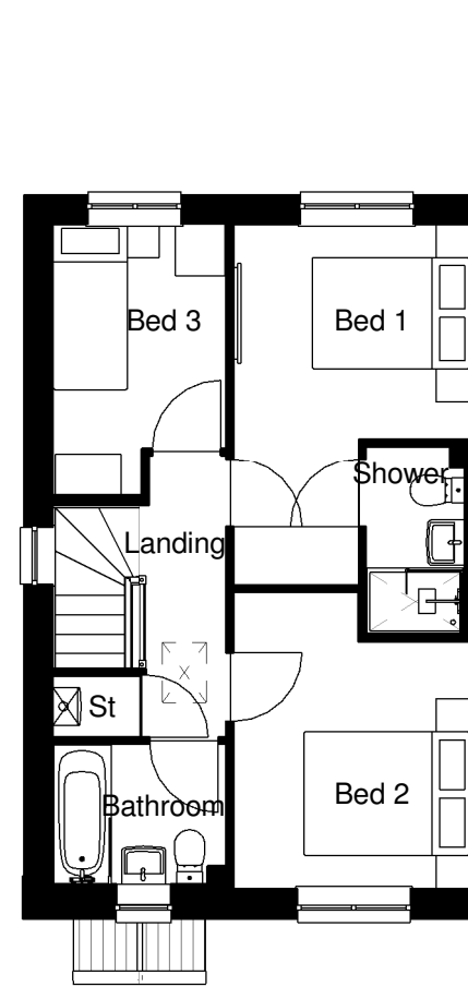
First Floor. 1 : 100
