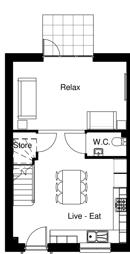
Ground Floor. 1 : 100
